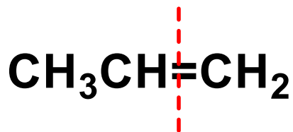
propen
