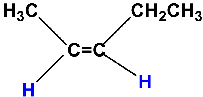
cis-2-penten
