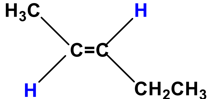
trans-2-penten
