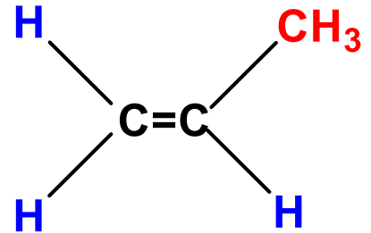
propen
