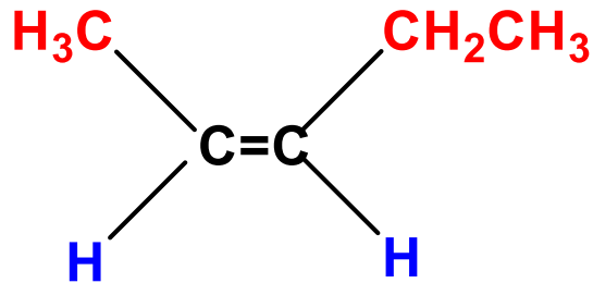
2-penten
